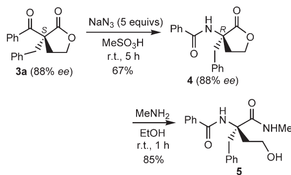
Scheme 2. Facile conversion of 3a to \alpha,\alpha -dialkyl- \alpha -amino acid derivatives 4 and 5 .
