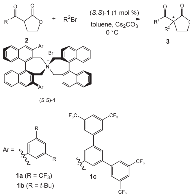
Scheme 1. Asymmetric alkylation of \alpha -acyl- \gamma -butyrolactones 2 under phase-transfer conditions using ( S,S )- 1 as catalyst.
